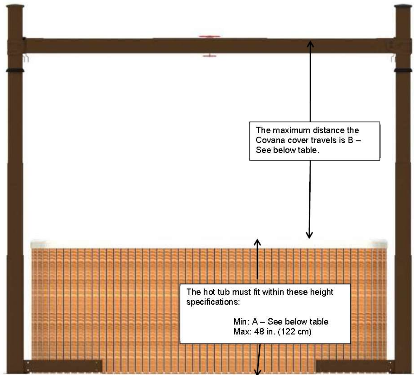
Covana Evolution - Side Elevation Dimensions
